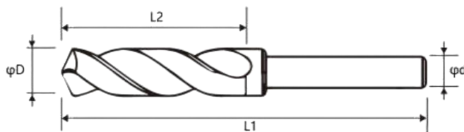
DRILL BIT
